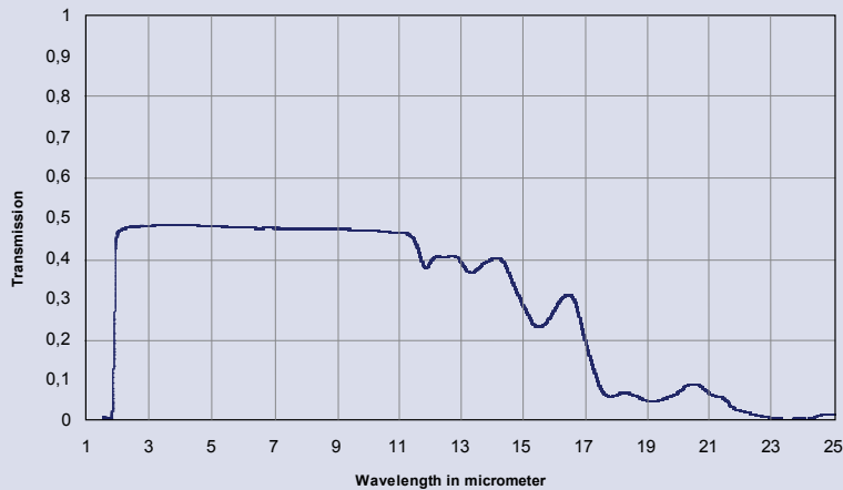
Transmission of Germanium at 23°C [3]
